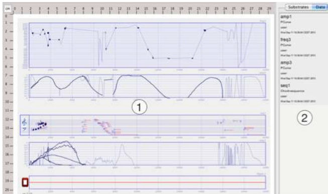
Figure 4: Polyphony interface with data from P3. (1) Virtual page with data from Max and digital pen. (2) List of available Max data streams.
