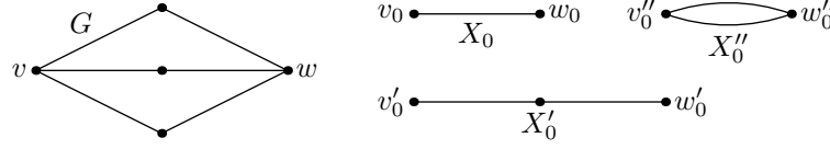
Fig. 4: A model graph G and three initial graphs X_0, X'_0, X''_0 .
