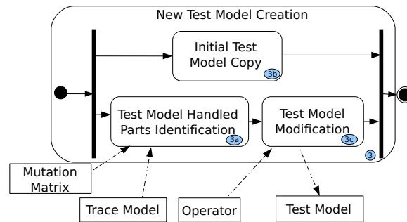
Figure 9. New Test Model Creation Process
