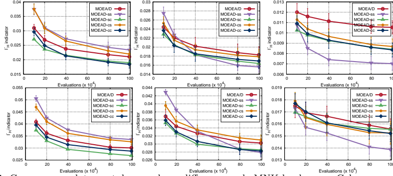
Fig. 1. Convergence plots w.r.t. hypervolume difference and \rho MKN-landscapes. Columns are respectively for \rho \in \{-0.7, 0.0, 0.7\} . Rows are respectively for K \in \{4, 8\} . Results are for \mu = 128 , T = 8 , \delta = 1.0 , cr = 1.0 , nr = 0 and g^{te} .
