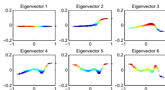
Figure 1. Eigenvectors from the Flixster data corresponding to the smallest few eigenvalues projected onto the first principal component. Colors indicate the values.
