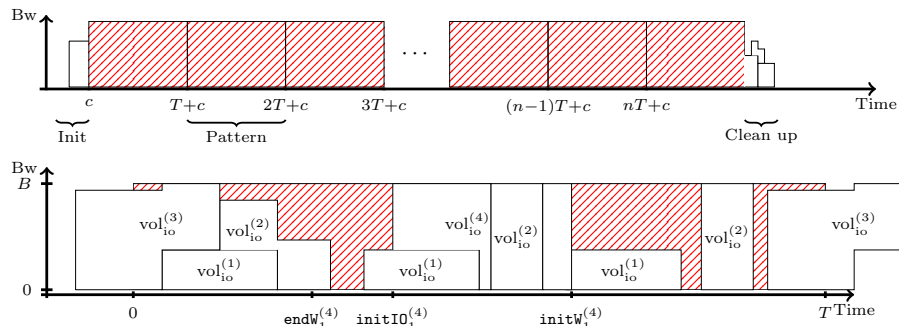
Figure 4: A periodic schedule (above), and the detail of one of its regular period (below) where (w^{(1)} = 3.5; \text{vol}_{\text{io}}^{(1)} = 240; n_{\text{per}}^{(1)} = 3) , (w^{(2)} = 27.5; \text{vol}_{\text{io}}^{(2)} = 288; n_{\text{per}}^{(2)} = 3) , (w^{(3)} = 90; \text{vol}_{\text{io}}^{(3)} = 350; n_{\text{per}}^{(3)} = 1) , (w^{(4)} = 75; \text{vol}_{\text{io}}^{(4)} = 524; n_{\text{per}}^{(4)} = 1) .
