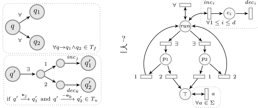
FIGURE 7. Reducing AVASS non-termination to a simulation FS \preceq BPP.
