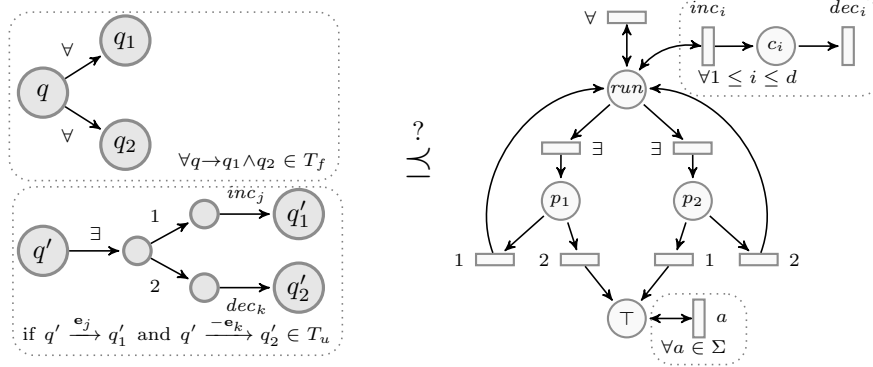
FIGURE 5. Reducing AVASS non-termination to a simulation \text{FS} \preceq \text{BPP} .
