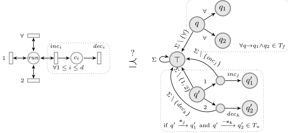
FIGURE 4. Reducing AVASS state reachability to a simulation \text{BPP} \not\leq \text{FS} .
