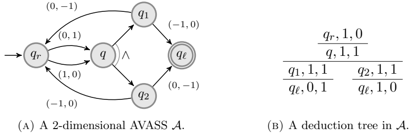
(A) A 2-dimensional AVASS \mathcal{A} .
