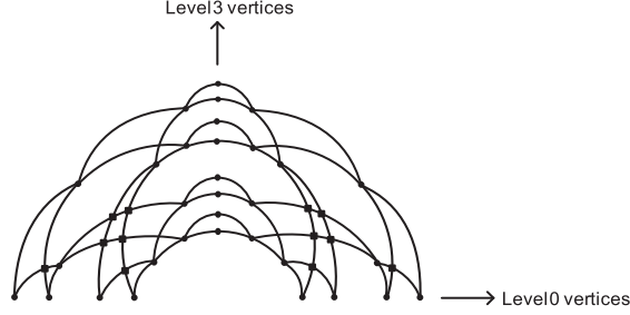
Fig. 3: Additional crossings in the formation of \phi'(BF_3)
