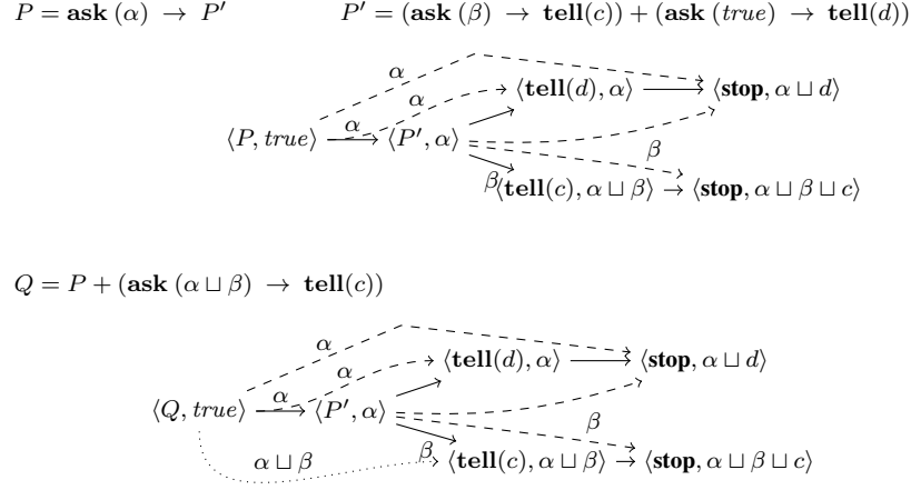
Figure 5: LTS_{\Rightarrow}(\{\langle P, true \rangle, \langle Q, true \rangle\}) where \Rightarrow is defined in Table 5 (Milner's saturation method). The cycles from rule MR2 are omitted. The dashed transitions are those added by the rules in Table 5. The dotted transition is the (irredundant) one that \langle Q, true \rangle can take but \langle P, true \rangle cannot match, therefore showing that \langle P, true \rangle \not\sim_I^{\Rightarrow} \langle Q, true \rangle
