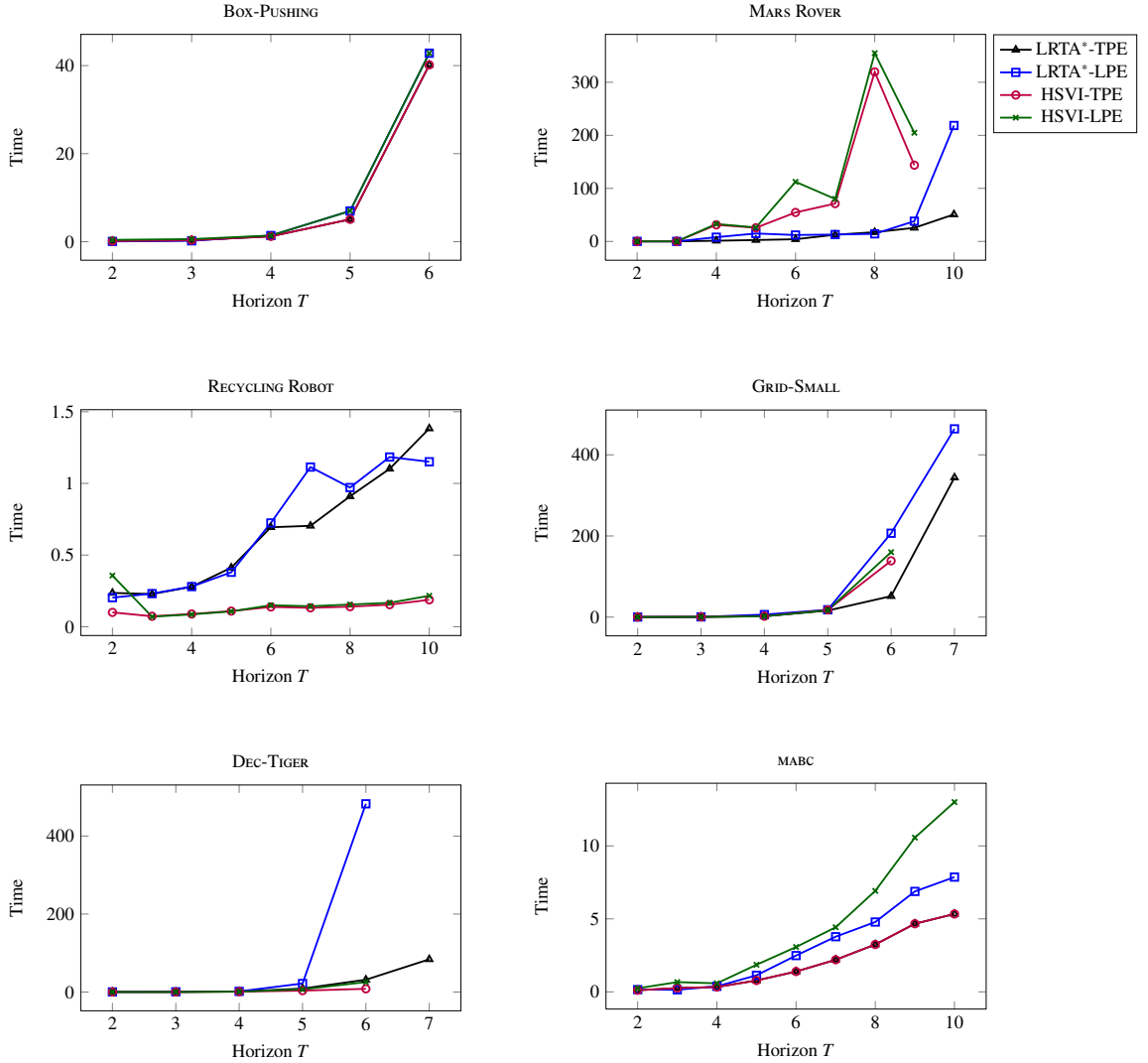
Figure 14: Comparison of compression methods to maintain concise data through LRTA^* , LRTA^* -TPE, HSVI-LPE, and HSVI-TPE. All graphs show the time required to convergence (in seconds) on the y -axis given the various planning horizons on the x -axis.
