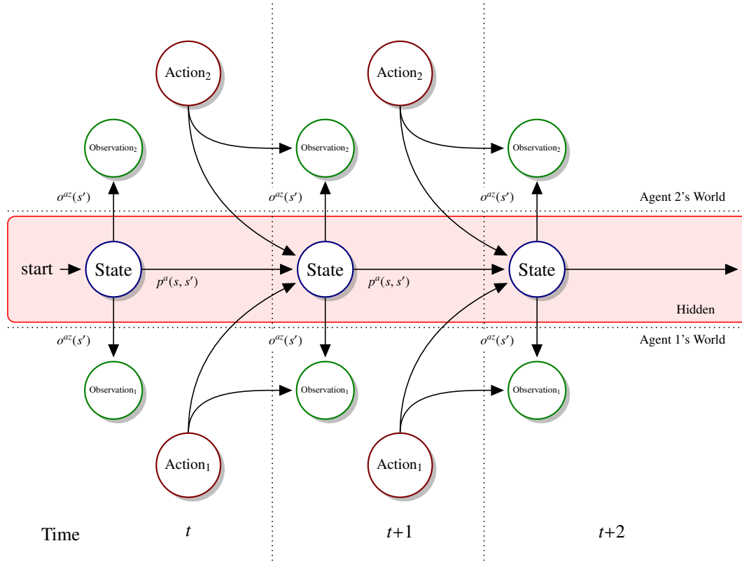
Figure 1: A graphical model of the two-agent Dec-POMDP model, where rewards are omitted
