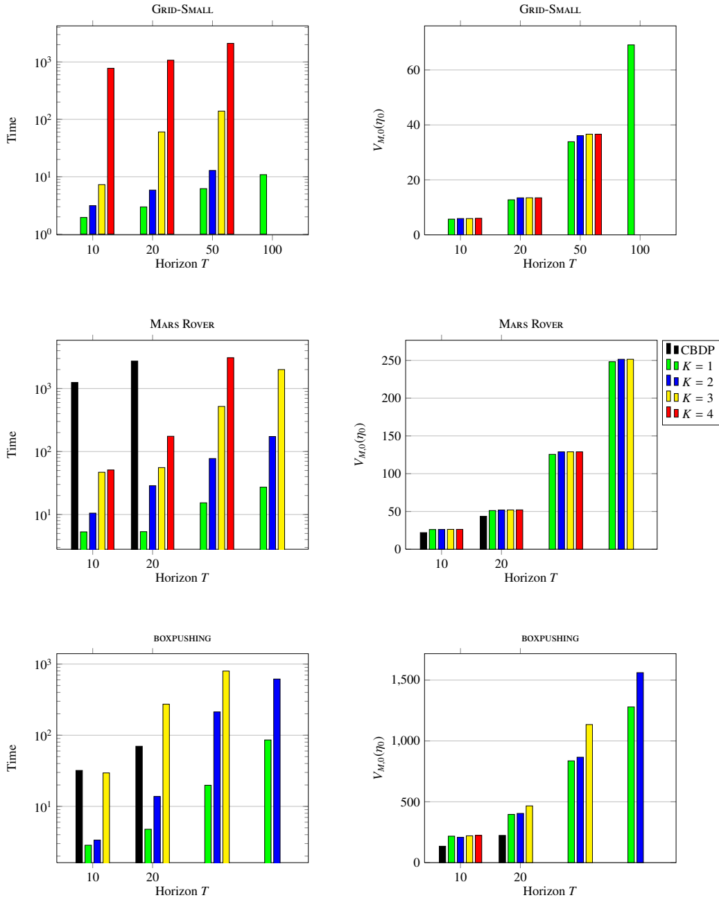
Figure 5: The performance of K -FB-HSVI and CBDP algorithms over our selection of benchmarks and larger planning horizons.
