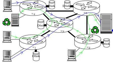
Figure 4: Request flows merge, split, move in opposite directions at some nodes.
