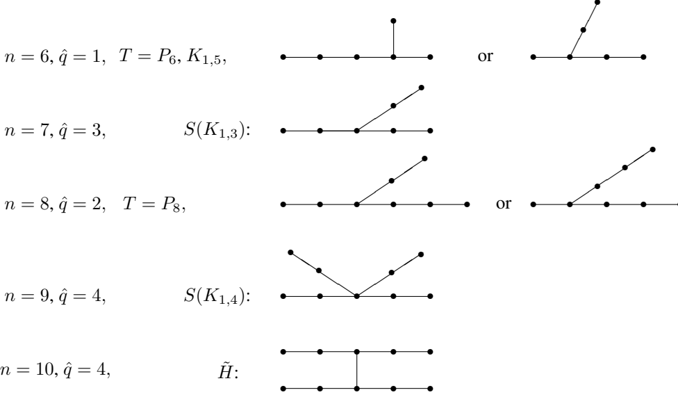
Fig. 1: All maximum n -vertex trees T with n \leq 10
