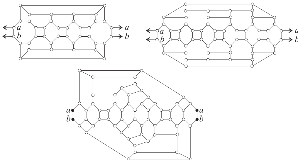
Fig. 7: The second graph from the twisted chamfered cube tribe, the second graph from the \mathcal{CI}(G_1) -tribe, and the graph on 60 vertices from the \mathcal{CI}(G_2) -tribe.
