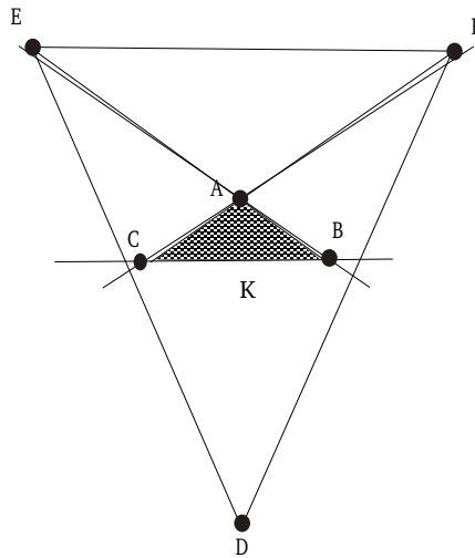
Fig. 23: ( 2I, O ) configuration
