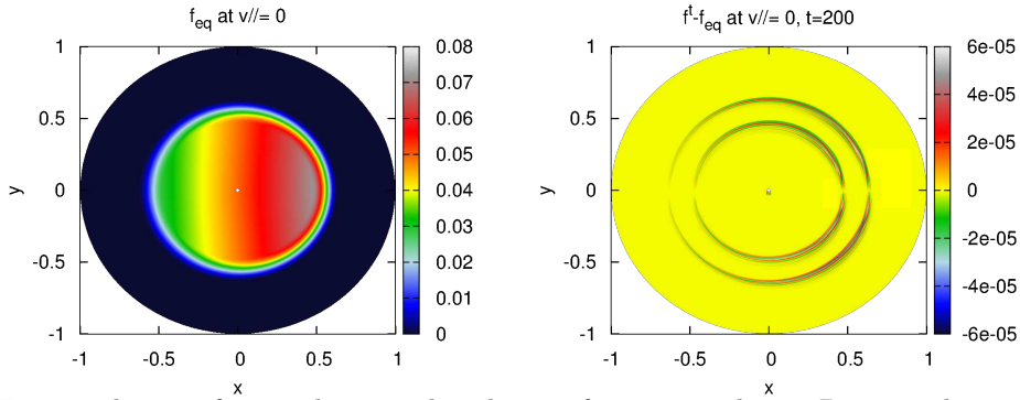
Figure 6: Time evolution of a steady state distribution function without 4D interpolation and without delta-f interpolation techniques, poloidal cut at v_\parallel = 0, \varphi = 0 (ideally f^t - f_{eq} remains zero)
