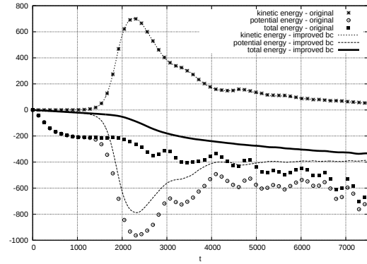
Figure 4: Evolution of the energies for a 4D toroidal test case, \mu = 3 .
