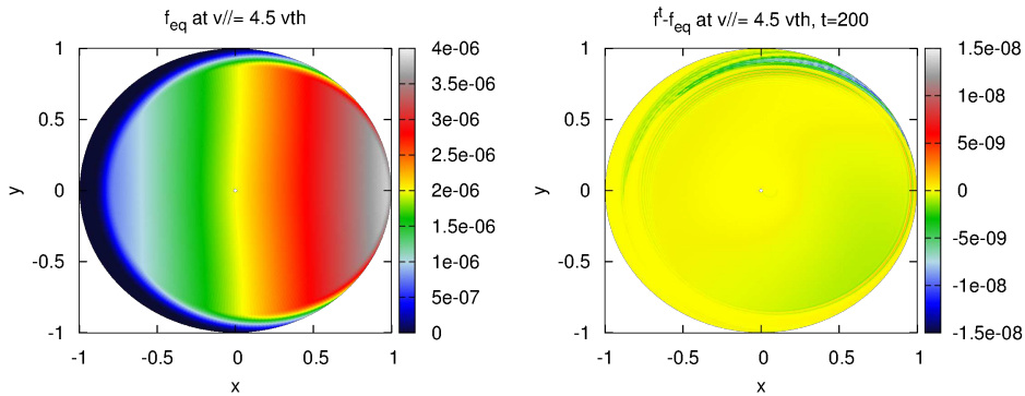
Figure 7: Time evolution of a steady state distribution function without 4D interpolation and without delta-f interpolation techniques, poloidal cut at v_\parallel = 4.5 v_{th}, \varphi = 0 (ideally f^t - f_{eq} remains zero)
