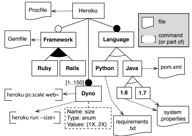
Figure 4: The Heroku FM and its Assets (excerpt)
