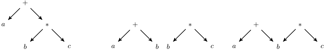
Figure 6: The directed graphs of a + b * c and a + b, b * c
