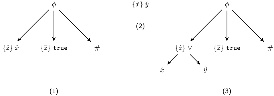
Figure 19: The graphs of (1) z := \hat{x} , (2) x \hat{=} y and (3) z := x \hat{+} y
