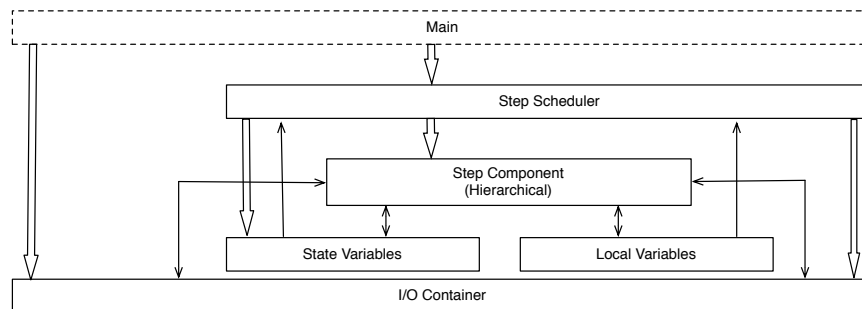
Figure 2: Code generation: General scheme
