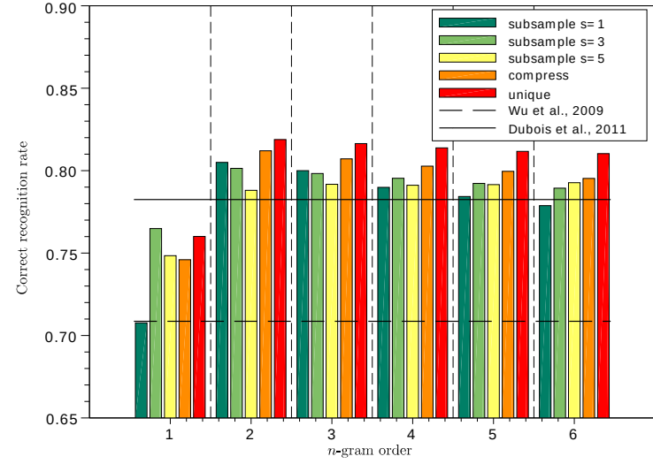
(b) S = 10 , Witten-Bell smoothing
