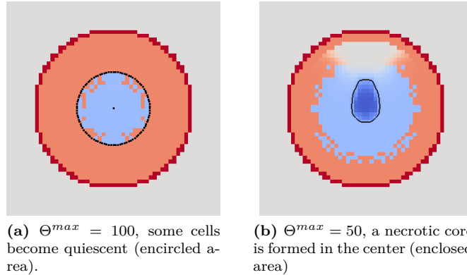
Figure 11: Nutrient influence: quiescent cells are in light blue and necrosis in dark blue ( t=11 ).
