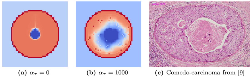
Figure 26: Simulation of the TNF effect on tumor necrosis ( t = 11 , \Lambda_\tau = 8 , D_\tau = 2 , \tau_{th} = 0.5 ).
