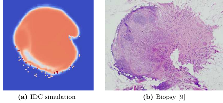
Figure 2: Main result : qualitative comparison of our simulation with biopsy.
