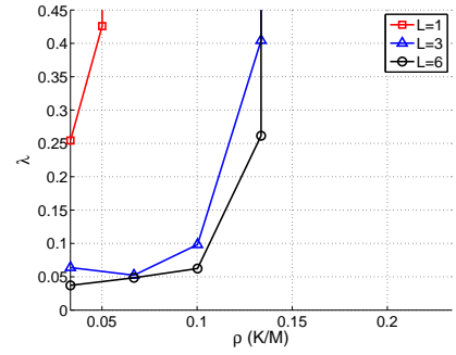
(a) Lower bound for \lambda , \delta = 0.6
