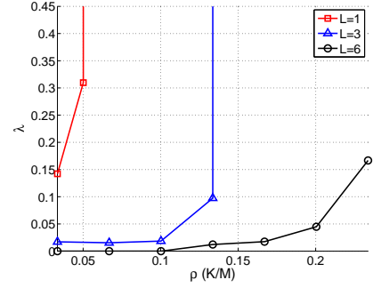
(b) Lower bound for \lambda , \delta = 1.2
