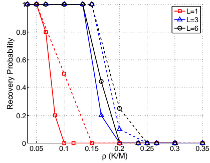
(c) Probability of recovery, \delta = 0.6
