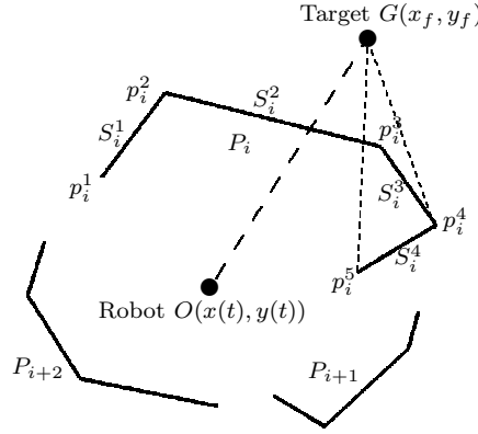
Figure 8. Intermediate objectives generation
