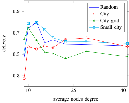
Fig. 15. Delivery ratio for NFP routing on SensLAB.
