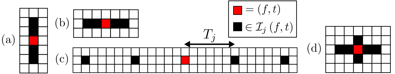
Fig. 1. Examples of proximity kernels to account for prior knowledge about sources. (a) vertical , for percussive elements, (b) horizontal , for stable harmonic elements, (c) periodic , for repetitive elements, (d) cross-like , for smoothly varying spectrograms such as vocals.
