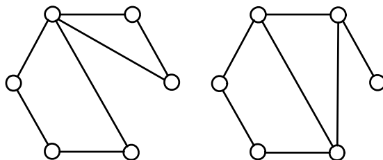
Fig. 6: Non-isomorphic graphs having the same generalized chromatic polynomial.
