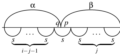
Fig. 14. The situation when |s| < |\beta^n| and n = 1 .
