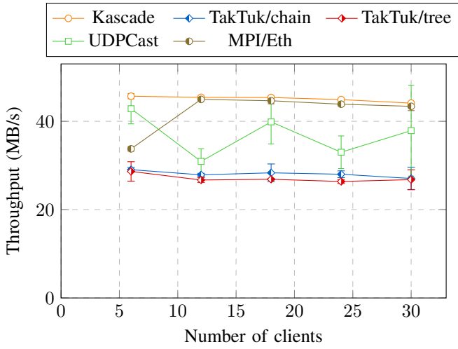
Fig. 11. The performance of the methods using 1 Gbit/s Ethernet network if the clients store the file on a hard disk. Kascade shows the best performance among the methods.
