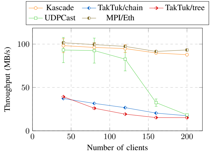
Fig. 7. Performance and scalability using up to 200 nodes on 1 Gbit/s Ethernet. Only Kascade and MPI Broadcast fully saturate the available bandwidth and scale very well with number of nodes.
