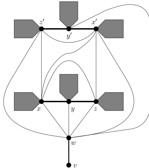
Figure 7: The forcing gadget with head v . (Edges of E(F) are in bold, no-3-gadgets are represented by their symbols.)
