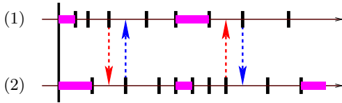
Figure 8. Synchronization principle used in time-based LTTA.
