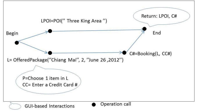
Fig. 3. Orchestration model with user interactions
