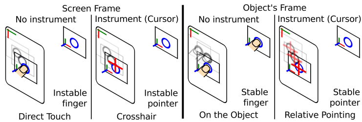
Fig. 3. Pointing through live video: four cases.
