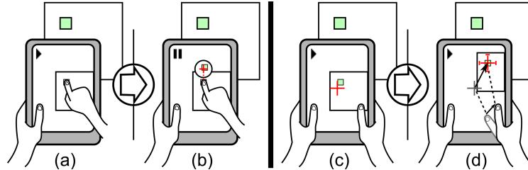
Fig. 1. Four techniques for pointing at physical objects through video on handheld devices: (a) Direct Touch on the live video; (b) Shift&Freeze : Shift [19] combined with freeze-frame; (c) Screen-centered Crosshair ; (d) Relative Pointing with cursor stabilized on the physical object.
