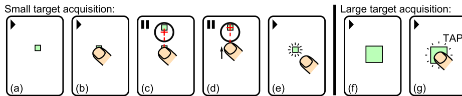
Fig. 4. Shift&Freeze walkthrough. (a-e) Small target acquisition with Shift and frozen video; (f-g) Large target acquisition with the Direct Touch technique (one tap on the screen).
