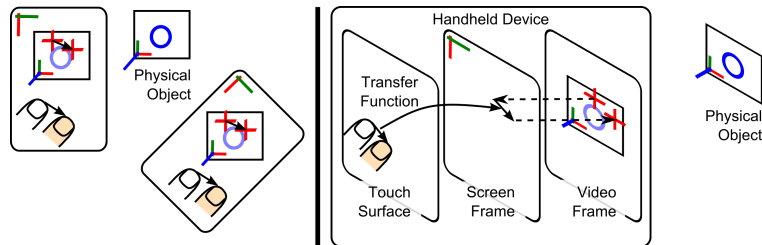
Fig. 6. With Relative Pointing : (left) Effect of screen rotation on the cursor's position; (right) The cursor is stabilized in the physical object's frame of reference and relative touch motions are applied on the screen.
