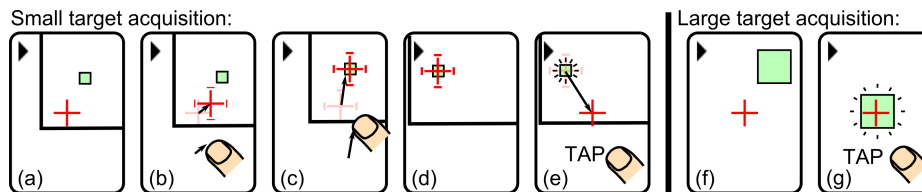
Fig. 5. Relative Pointing walkthrough. (a-e) Small target acquisition with a relative cursor stabilized on the physical object; (f-g) Large target acquisition with the crosshair technique.
