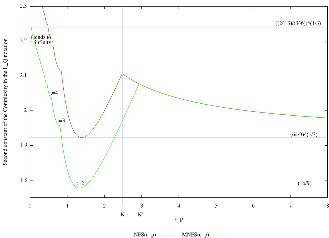
Figure 4: Asymptotic complexities L_Q(1/3, \text{NFS}(c_p)) or L_Q(1/3, \text{MNFS}(c_p)) in the boundary case, as a function of c_p with p = L_Q(2/3, c_p) . The red curve corresponds to the classical variants of NFS and NFS-HD, while the green dotted one corresponds to MNFS. The crossing point between NFS-HD and NFS, which is given by c_p = K \approx 2.5 in the classical NFS, switches to c_p = K' \approx 2.9 in MNFS. Here t is the number of terms (degree t - 1 ) of the polynomials in the sieving space.
