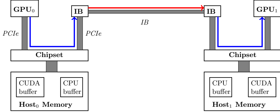
Fig. 6: Data copy from GPU 0 to GPU 1 with Cuda-aware MPI and GPU Direct
