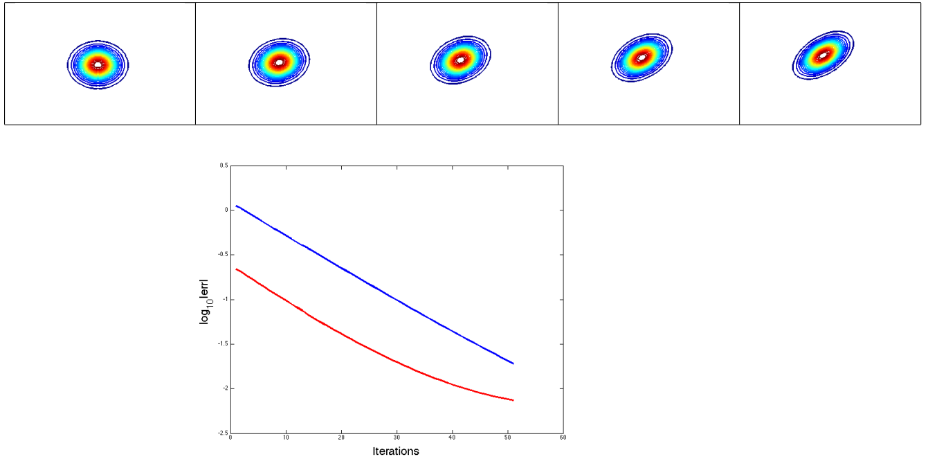
Figure 2: TC1. Top picture row: plot of density isolines \rho(t, x) for t = 0, 0.25, 0.5, 0.75, 1 along with the optimal path computed by algorithm 2. Bottom: red (resp. blue) line represents the error in L^1 norm (resp. L^\infty norm).
