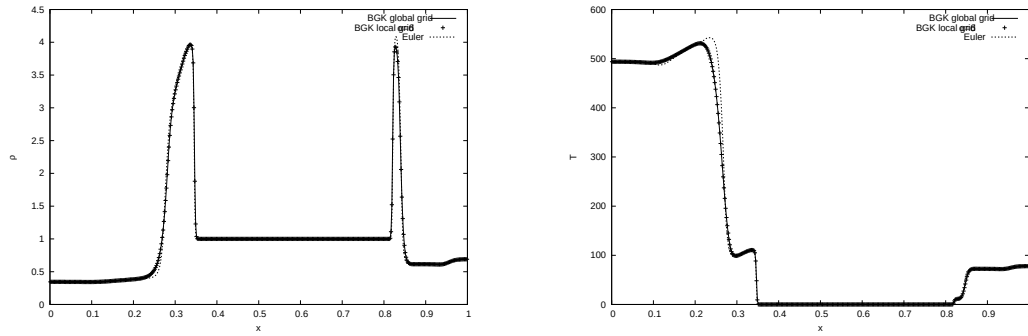
Figure 3: Test case 1, Kn = 10^{-5} : Density (left) and temperature (right) solution with 500 grid points in space
