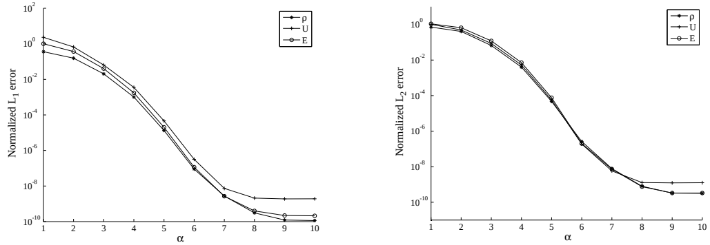
Figure 5: Test case 1, Kn = 10^{-5} : L_1 (left) and L_2 (right) error on density, velocity and energy
