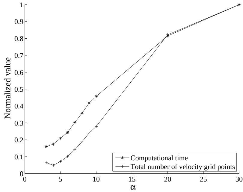
Figure 19: Test case 2, Kn = 10^{-2} : Normalized number of velocity grid points used and computational time with respect to the full grid calculation
