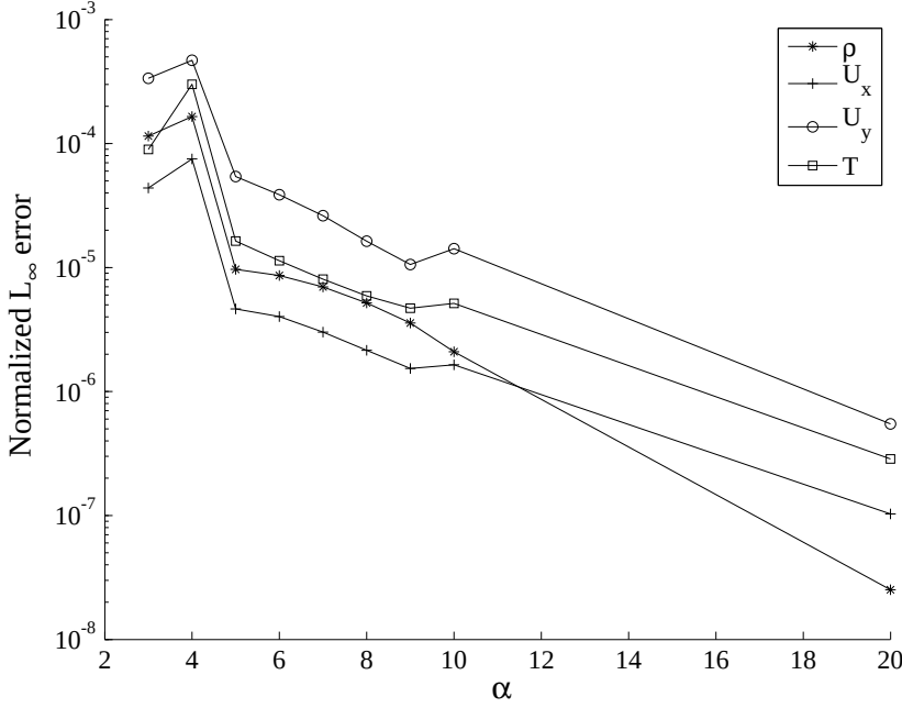
Figure 18: Test case 2, Kn = 10^{-2} : L_\infty error on density, velocity and temperature
