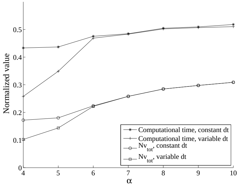
Figure 9: Test case 1, Kn = 10^{-5} : Normalized number of velocity grid points used and computational time with respect to the global grid calculation
