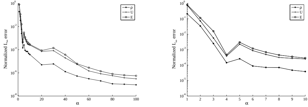
Figure 10: Test case 1, Kn = 10^{-2} : L_\infty error on density, velocity and energy (left) with a zoom on small values of \alpha (right)
