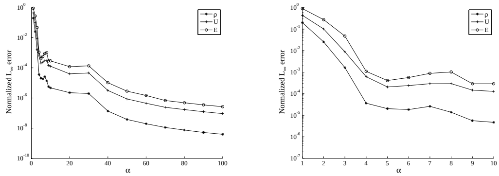
Figure 11: Test case 1, Kn = 1 : L_\infty error on density, velocity and energy (left) with a zoom on small values of \alpha (right)
