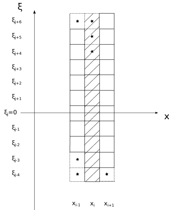
Figure 1: Representation of velocity-space cells in phase space in 1D. Local grids defined in cell i - 1, i, i + 1 before the union are in solid lines and stencil used for the transport in space cell i after the union is in dashed lines. Cells in the local grid for space cell i are hatched. Cells with marker ★ are cells added after the union.
