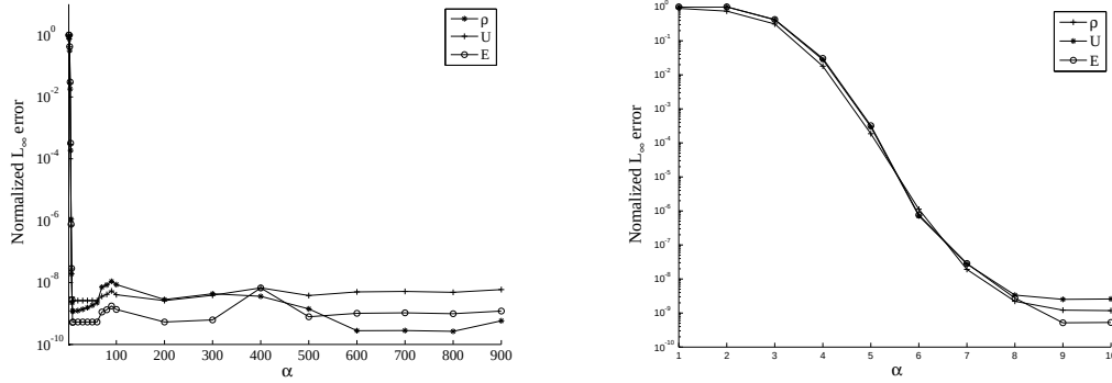
Figure 6: Test case 1, Kn = 10^{-5} : L_\infty error on density, velocity and energy
