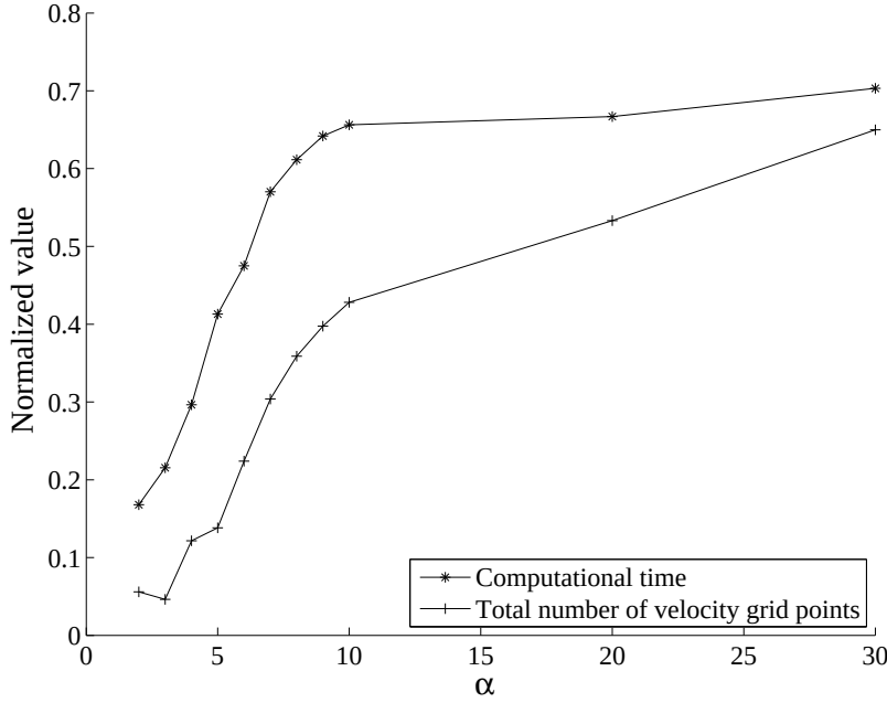
Figure 21: Test case 3, Kn = 10^{-5} : Normalized number of velocity grid points used and computational time with respect to the full grid calculation
