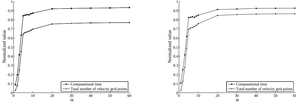
Figure 12: Computational time and total number of velocity grid points used for Kn = 10^{-2} (left) and Kn = 1 (right)
