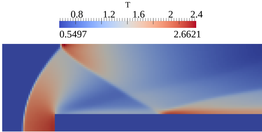
Figure 13: Solution for the temperature ( Kn = 10^{-5} )
