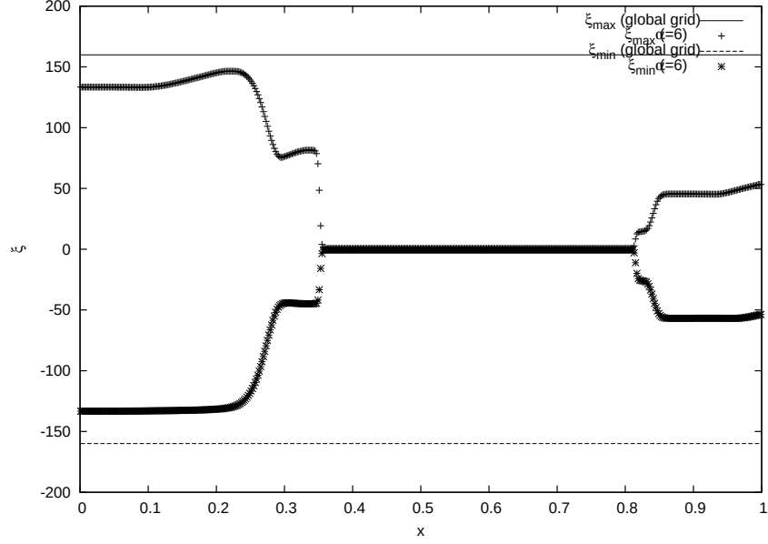
Figure 4: Test case 1, Kn = 10^{-5} : Maximum and minimum velocity in the local grid for \alpha = 6
