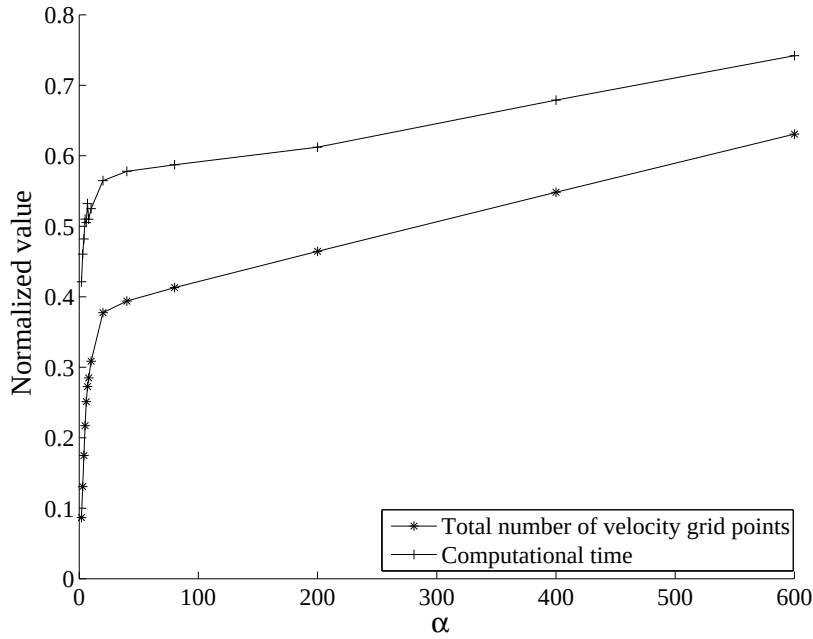
Figure 8: Test case 1, Kn = 10^{-5} : Normalized number of velocity grid points used and computational time with respect to the global grid calculation
