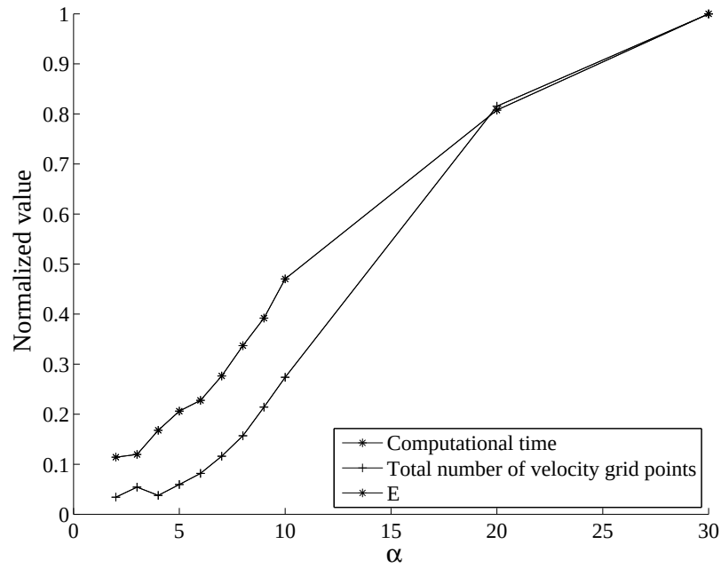
Figure 16: Normalized number of velocity grid point used and computational time with respect to the full grid calculation ( Kn = 10^{-5} )
