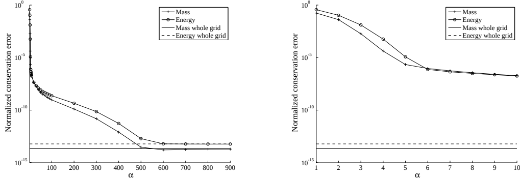
Figure 7: Test case 1, Kn = 10^{-5} : Conservation error
