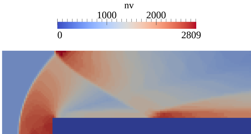
Figure 17: Number of velocity grid points used in each cell at t=1.2 for \alpha = 10 ( Kn = 10^{-5} )
