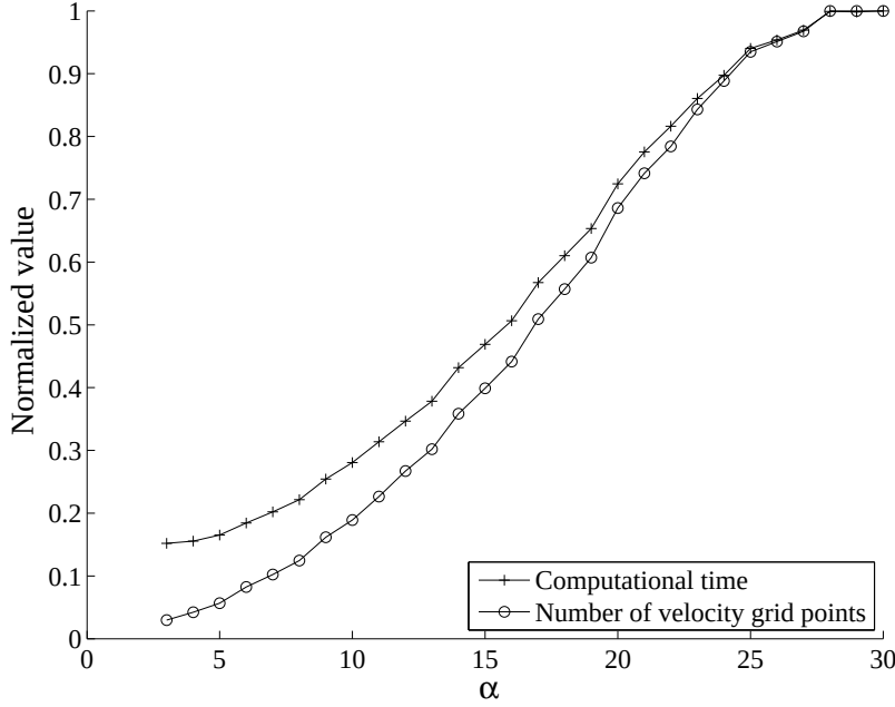
Figure 15: Normalized number of velocity grid point used and computational time with respect to the full grid calculation for one iteration on one processor ( Kn = 10^{-5} )
