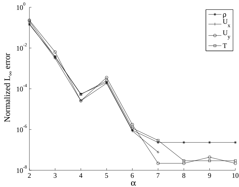
Figure 20: Test case 3, Kn = 10^{-5} : L_\infty error on density, velocity and temperature
