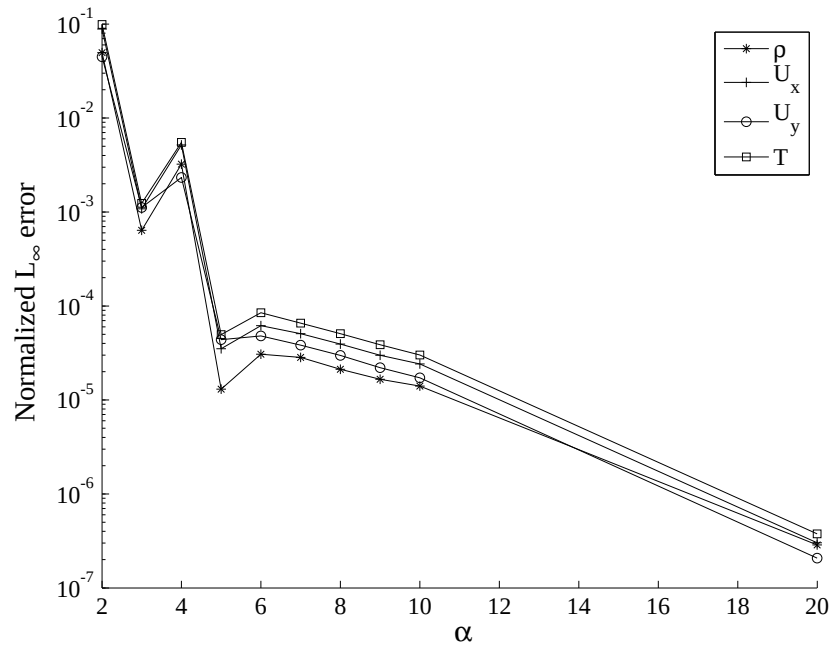
Figure 14: Test case 2, Kn = 10^{-5} : L_\infty error on density, velocity and temperature
