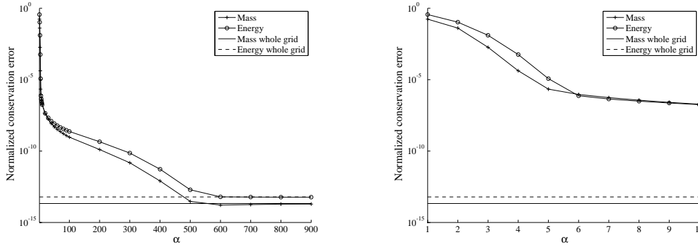
Figure 7: Test case 1, Kn = 10^{-5} : Conservation error
