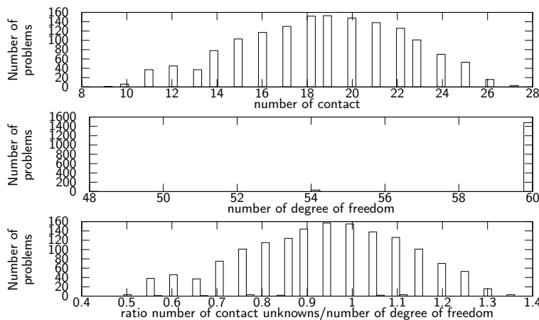
Figure 2: distribution of the number of contacts, the number of d.o.f and their ratio
