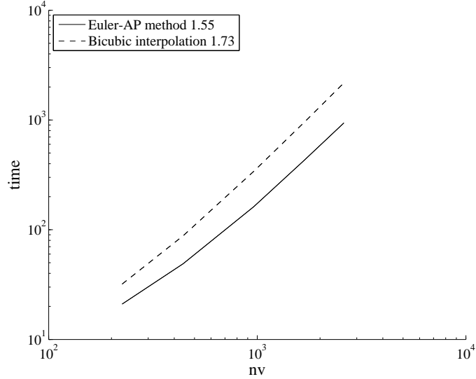
Figure 13: Computational time for the two methods with respect to the number of velocity grid points.
