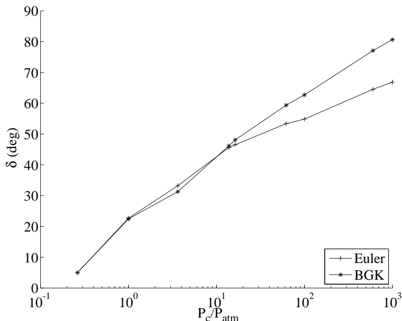
Figure 23: Angle for different pressure ratios calculated with Euler and BGK models.
