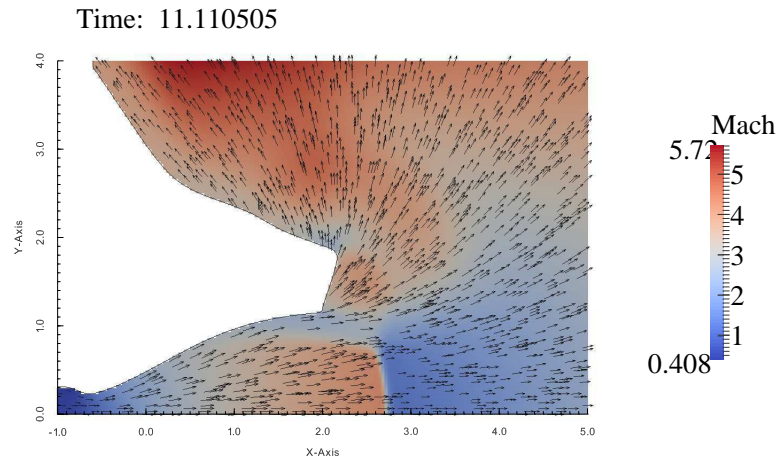
Figure 21: Mach number and velocity vectors at t=11 for P_c/P_{atm} = 2000 .
