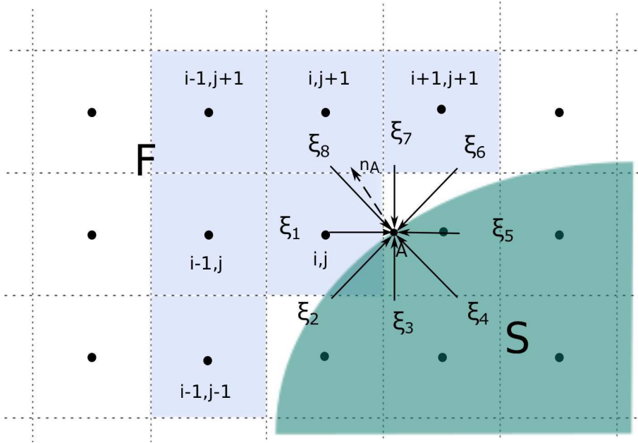
Figure 2: Graphic illustration of the reconstruction for a 8 velocities grid.
