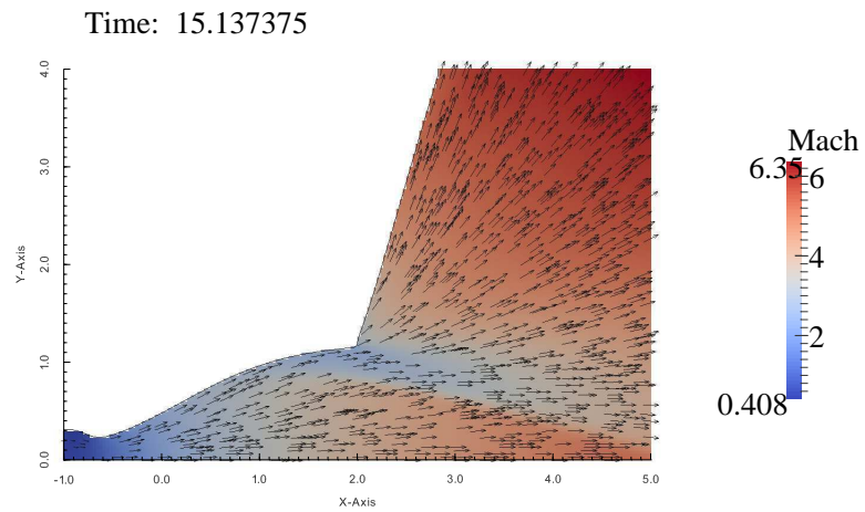
Figure 22: Mach number and velocity vectors at steady state for P_c/P_{atm} = 2000 .
