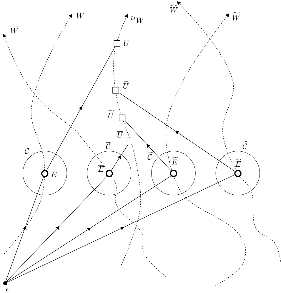
Figure VIII.6. The event e in the four past null cones of the four events E, \bar{E}, \tilde{E} and \hat{E} . This event e is observed on their respective celestial spheres \mathcal{C}, \bar{\mathcal{C}}, \tilde{\mathcal{C}} and \hat{\mathcal{C}} .
