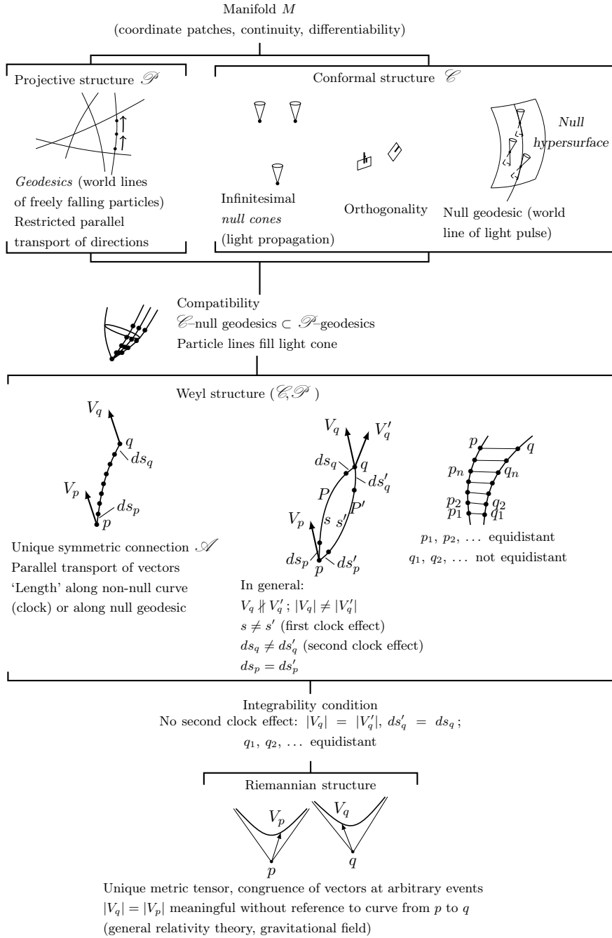
Figure II.1. General scheme of conformal, projective, Weyl, and Riemannian structures (From FIG. 1. in Ehlers-Pirani-Schild paper [EPS72, p.66])
