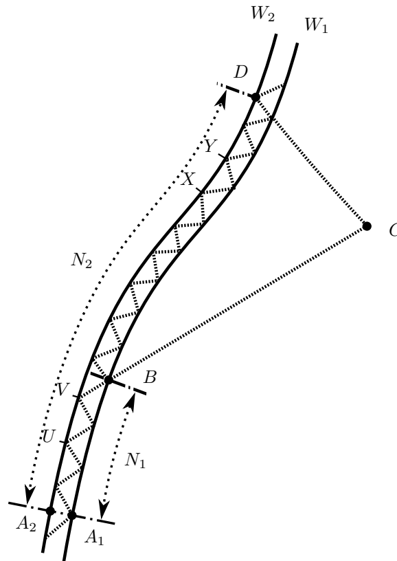
Figure A.1. Protocole de Marzke-Wheeler.
