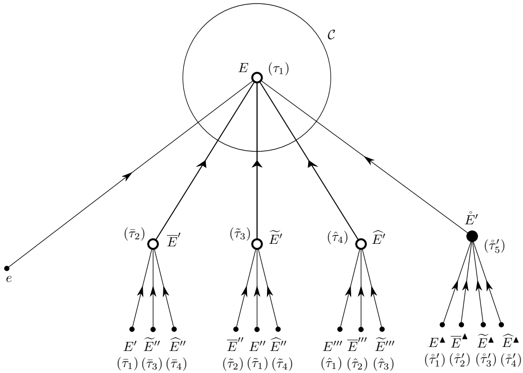
Figure VIII.7. The event E in the five future null cones of the five events e , \bar{E}' , \tilde{E}' , \hat{E}' and \overset{\circ}{E}' .
