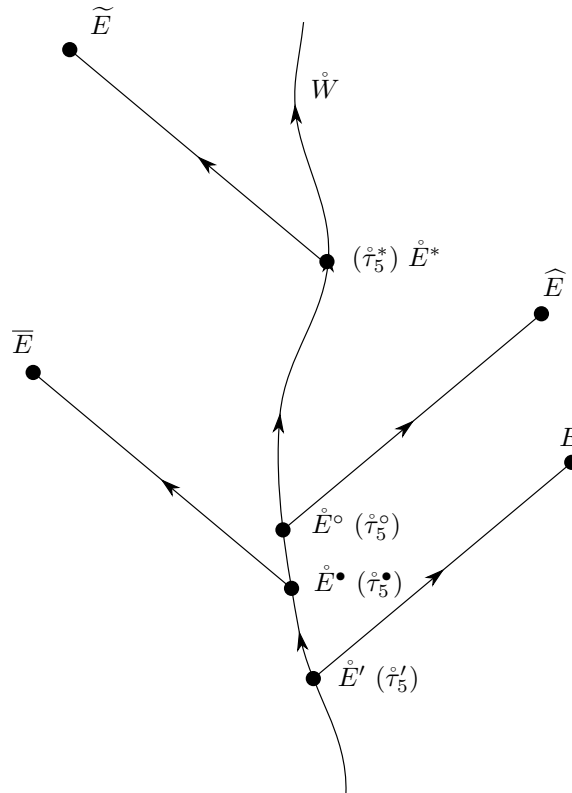
Figure VIII.8. An example of successive events \overset{\circ}{E}' , \overset{\bullet}{E} , \overset{\circ}{E}^\circ and \overset{\circ}{E}^* on the anchoring worldline of \overset{\circ}{\mathcal{E}} broadcasting their coordinates \overset{\circ}{\tau}_5 towards the four events E , \overline{E} , \widehat{E} and \widetilde{E} .
