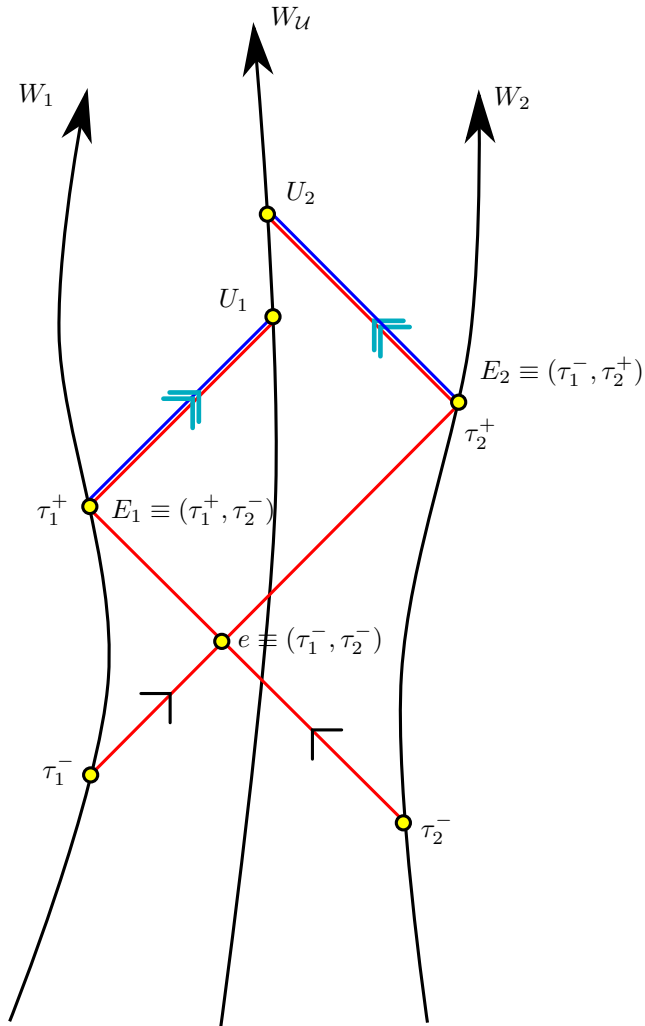
Figure VIII.1. The system of echoes in dimension two.
