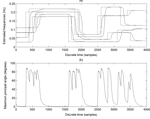
Fig. 2. OPAST / ESPRIT tracking: (a): Frequency tracking; (b): Maximum principal angle trajectory.
