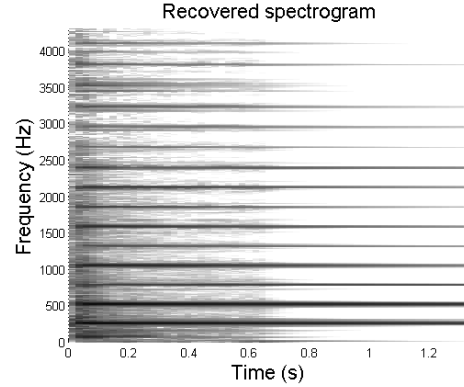
Figure 3: Recovery of the full C4 piano tone
