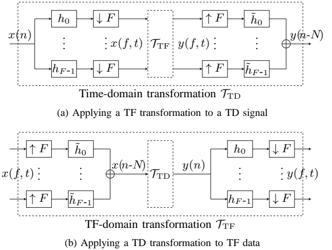
Fig. 1. Time-frequency vs. time domain transformations
