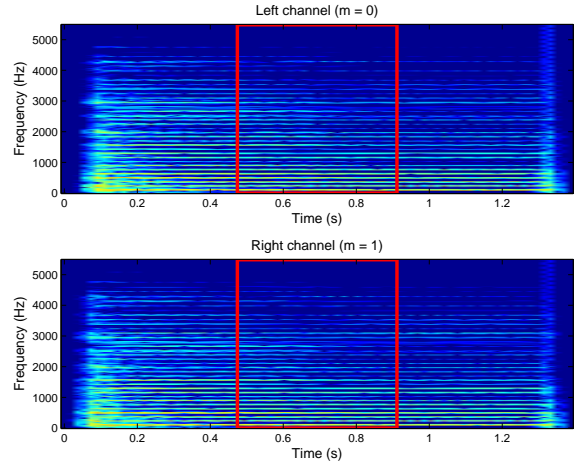
Fig. 3. Input stereo signal y_m(f, t) .
