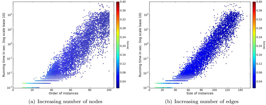
Figure 2: Computation time for Rome graphs. One dot per instance. The color indicates the density of the instance.
