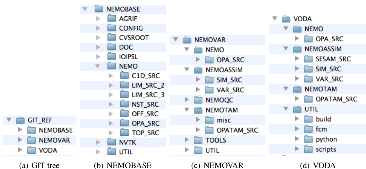
Figure 2.1: Code organization
