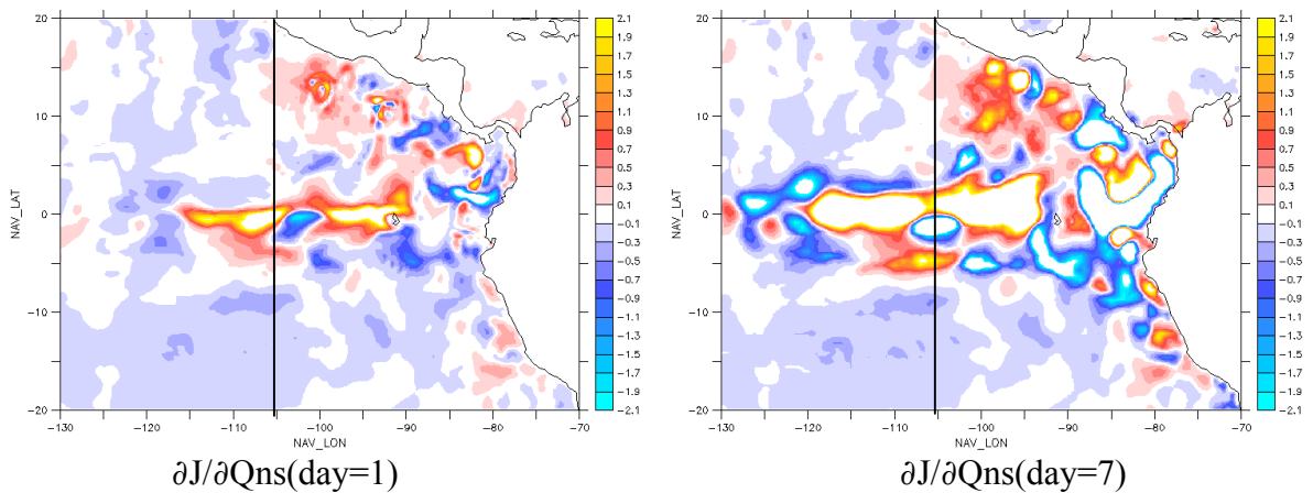
Figure 8: SST misfit sensitivity to heat flux of the first and last days
