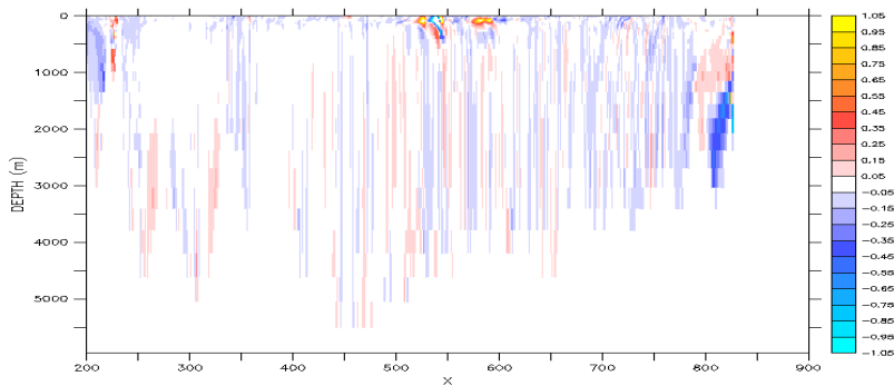
Figure 13: vertical section of \partial J(\text{SLA})/\partial T at 175^\circ\text{W}
