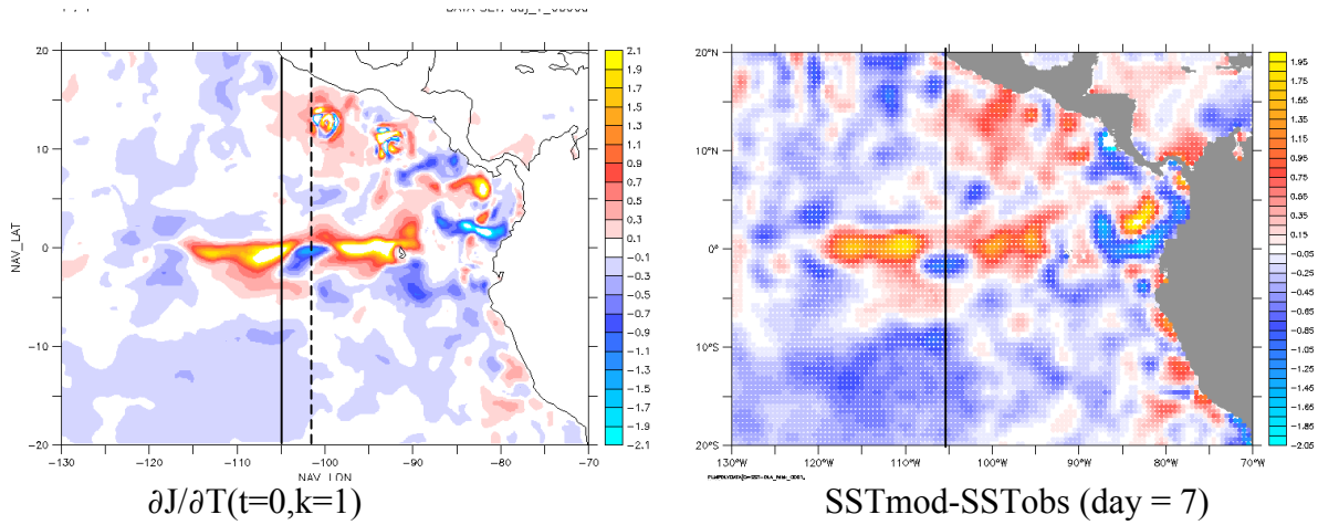
Figure 6: SST sensitivity to surface initial temperature, on the left, SST misfit on the day 7, on the right.
