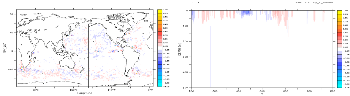
Figure 4: initial temperature sensitivity for J at 150m, weighted by the thickness of the grid level and a vertical section at 175°W
