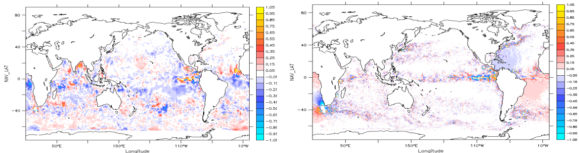
Figure 3: initial temperature and salinity sensitivity for J at the surface weighted by the thickness of the grid cell
